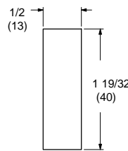
W6045 – Head Jamb Filler, Picture
