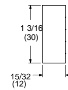
W6200 – Sill Liner, Picture
