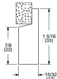
W7124 – Sill Liner w/ Adhesive Foam
